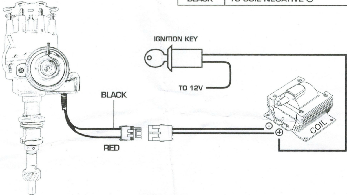
Wiring the Ready-to-Run Distributor.
